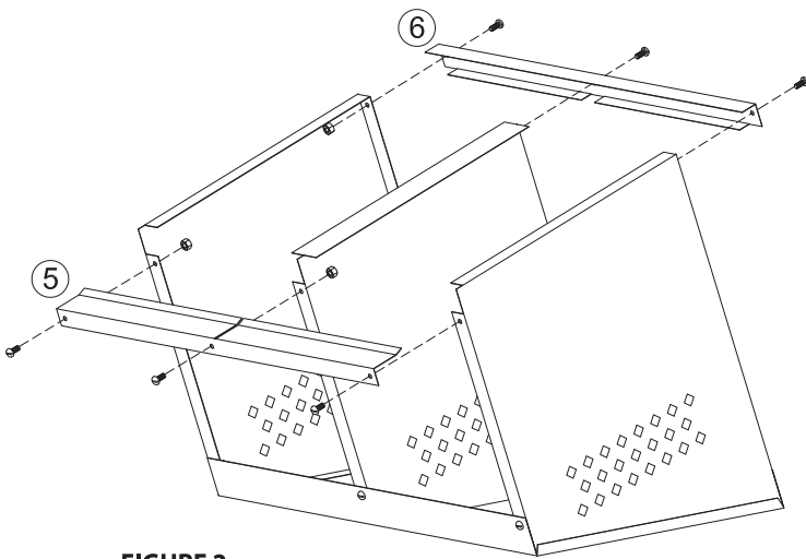
FIGURE 2 Fit the front and rear cross braces to the panels as shown, and screw into place
