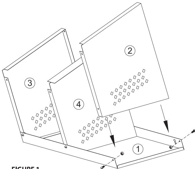
FIGURE 1 Mount the right and left side end panels and two division panels as shown and screw into place
