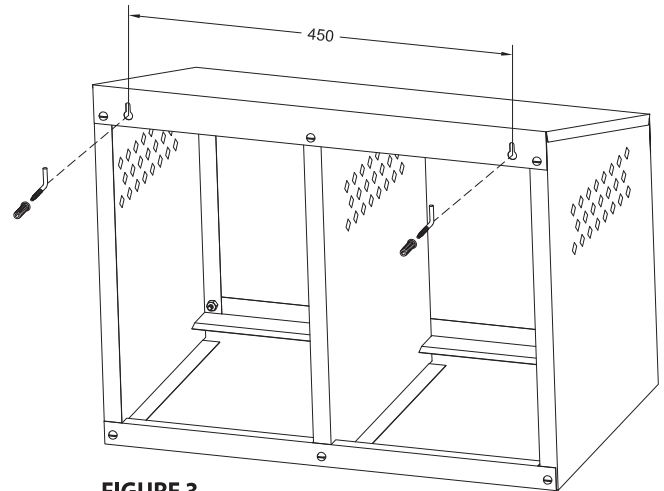
FIGURE 3 Mark the holes on the mounting surface using the nesting box as a template
